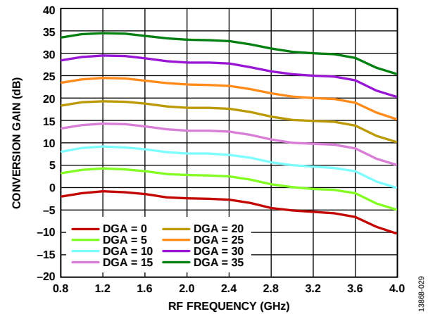
Figure 30. Conversion Gain vs. RF Frequency over DGA Word, Measurement Conducted with V_{CC\_VGA} = 3.3\text{ V} (Maximum Gain) on RF VGA
