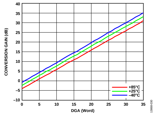
Figure 31. Conversion Gain vs. DGA Word over Temperature, Measurement Conducted with V_{CC\_VGA} = 3.3\text{ V} (Maximum Gain) on RF VGA, RF = 2 GHz
